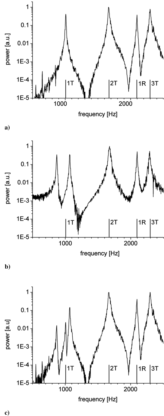
Fig. 7 Resonances of the CRC: a) without absorber, b) with absorber of length L/R = 0.85 and \alpha = 0 deg, and c) with absorber of length L/R = 0.85 and \alpha = 22.5 deg.
