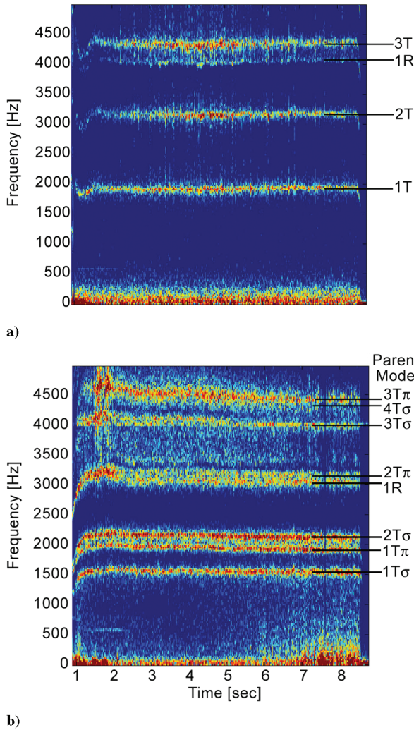
Fig. 6 Spectrogram of combustion noise: a) in CRC with no lateral cavity; b) with a lateral cavity placed at 135 deg with respect to the injector.
